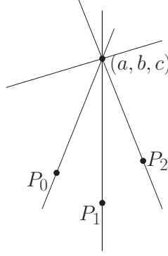
FIGURE 1. Quartic with a quadruple point
