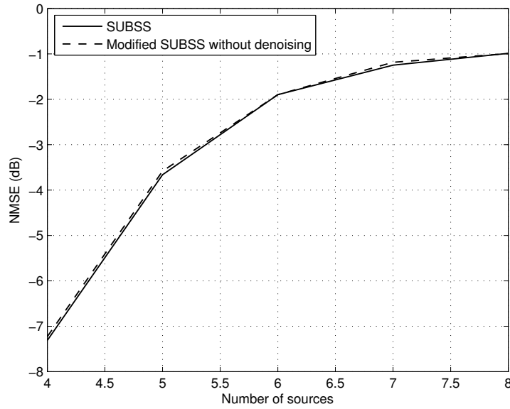
Fig. 8. Comparison between SUBSS and modified SUBSS without denoising when input SNR = 10dB: NMSE versus number of sources.
