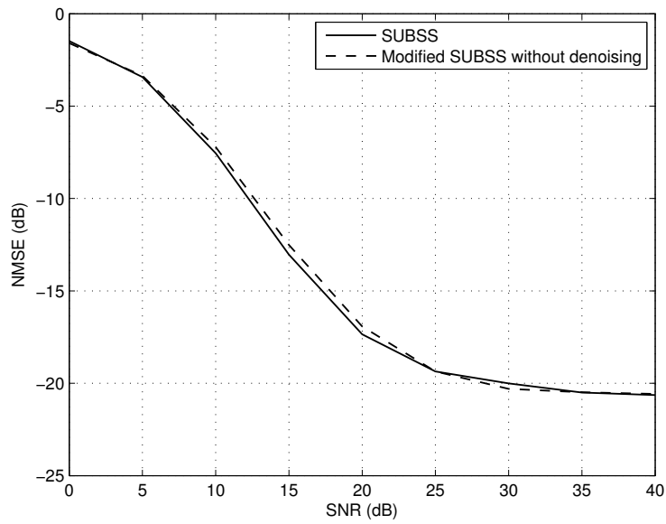
Fig. 12. Comparison of performance between SUBSS and modified SUBSS without denoising for chirp signals: NMSE versus SNR.
