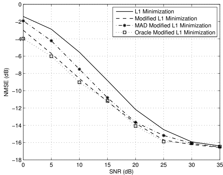
Fig. 14. Comparison of performance (NMSE versus SNR) between the original Bofill and Zibulevsky's method based on the \ell_1 -criterion of Eq. (4) (L1 Minimization), the modified \ell_1 -criterion of Eq. (14) after multisource selection when: the noise standard deviation is known (Oracle Modified L1 Minimization) or estimated via either the DATE (Modified L1 Minimization) or the MAD (MAD Modified L1 Minimization).
