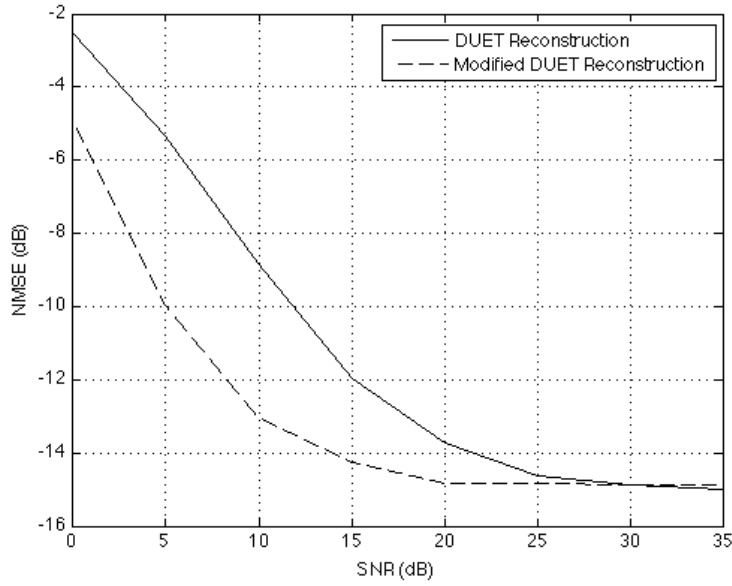
Fig. 15. Comparison of performance between DUET reconstruction and Modified DUET reconstruction on chirp signals
