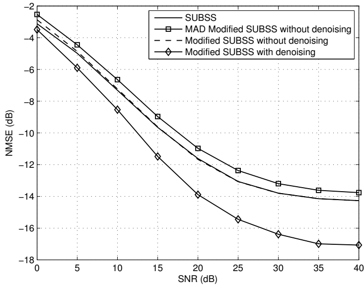
Fig. 7. Comparison between SUBSS, modified SUBSS with and without denoising, modified SUBSS with MAD estimate instead of DATE and without denoising: NMSE versus SNR.
