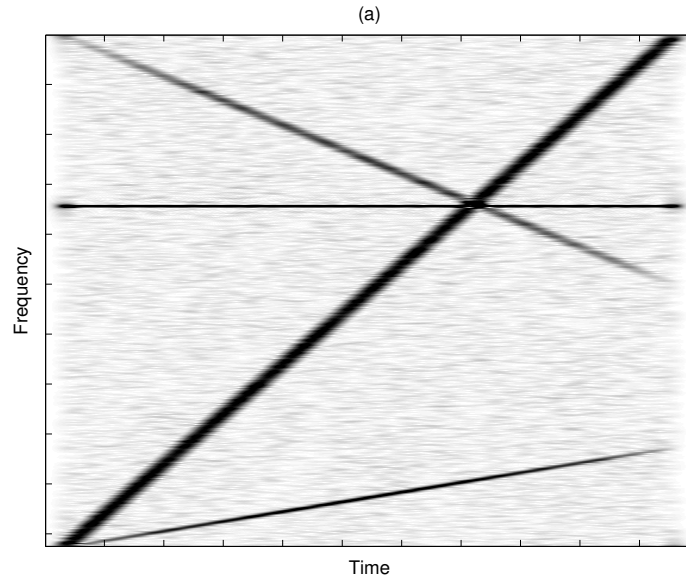
Fig. 11. Chirp signal mixture spectrogram when mixing matrix A is applied to the chirp signals of Figure 10 (SNR= 10dB).
