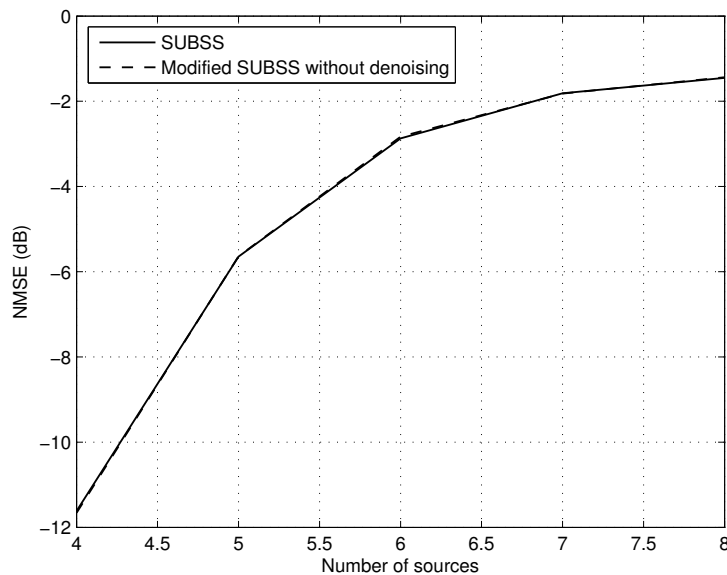
Fig. 9. Comparison between SUBSS and modified SUBSS without denoising when input SNR = 20dB: NMSE versus number of sources.
