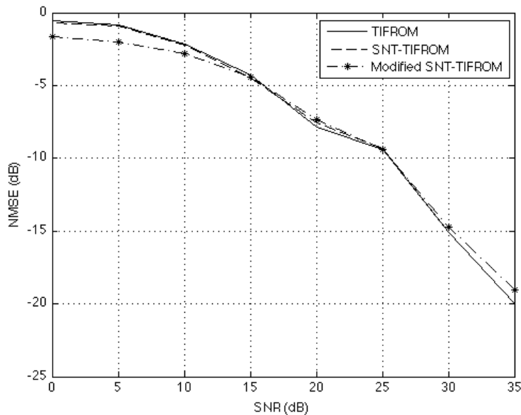
Fig. 13. Comparison of performance between TIFROM, SNT-TIFROM and Modified TIFROM: NMSE versus SNR.
