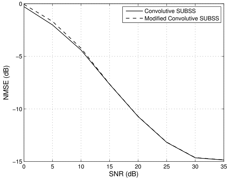
Fig. 16. Comparison of performance between standard convolutive SUBSS and modified convolutive SUBSS: the signals used are same audio one as those considered in Simulation Section. Each mixture is a sum of filtered source signal where each filter is randomly chosen RIF with order 4.
