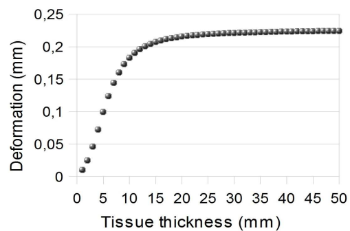
Figure 2 Deformation computed by 2D model as a function of tissue thickness (E=55kPa, P=20mbar)
