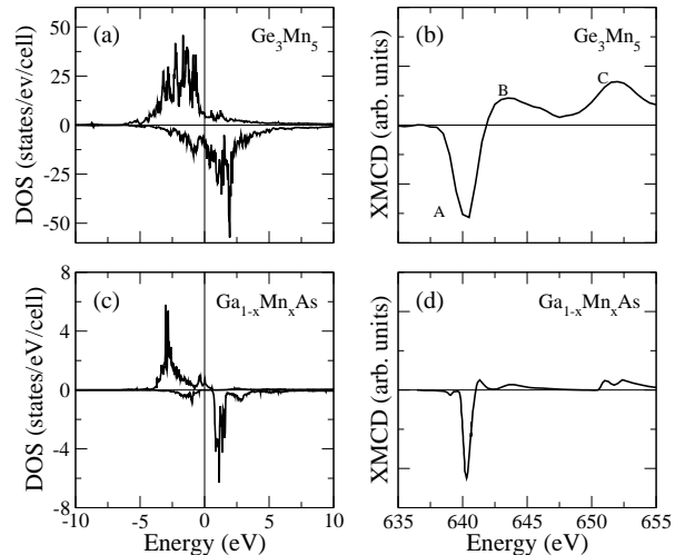
FIG. 3: 3d -states of Mn in (a) Ge 3 Mn 5 and (c) Ga 1-x Mn x As ( x=0.125 ). Experimental XMCD spectra at the L 2,3 edges of Mn in (b) Ge 3 Mn 5 (from Ref. 33) and (d) Ga 1-x Mn x As ( x=0.084 , from Ref. 51).
