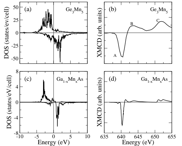
FIG. 3: 3d -states of Mn in (a) \text{Ge}_3\text{Mn}_5 and (c) \text{Ga}_{1-x}\text{Mn}_x\text{As} ( x=0.125 ). Experimental XMCD spectra at the L_{2,3} edges of Mn in (b) \text{Ge}_3\text{Mn}_5 (from Ref. 32) and (d) \text{Ga}_{1-x}\text{Mn}_x\text{As} ( x=0.084 , from Ref. 50).
