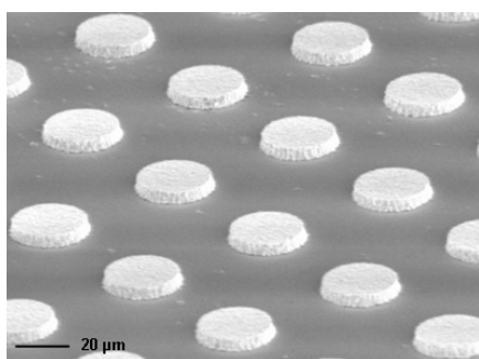
Figure 3: SEM view of the electroplated gold dots.
