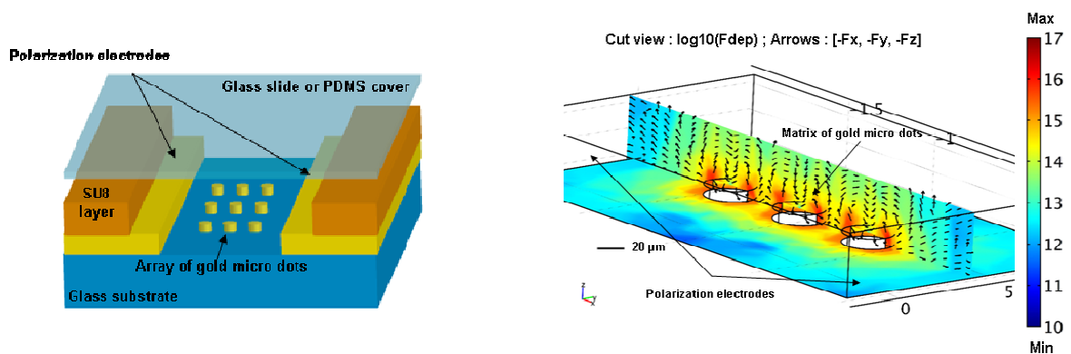
Figure 2: Finite element analysis of the DEP force ( F_{DEP} ) in the microfluidic channel.
