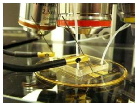
Figure 4: View the microfluidic chip under the microscope.
