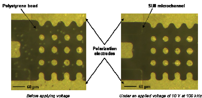
Figure 5: Gold dots and particles within the fluidic chip: particles are arrayed under an applied voltage of 10 V at 100 kHz.
