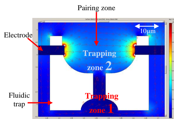
Figure 2: Comsol© simulation of the Electric field within the trap zone
