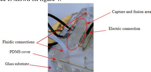
Figure 4: Packaged and connected electrofusion biochip
