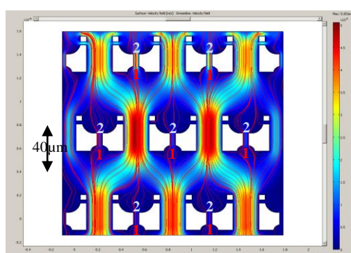
Figure 1: Comsol© simulation of the flow induced through the fluidic traps
