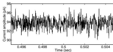
Figure 4: Real current variations through \alpha -hemolysin channel without any translocation event.
