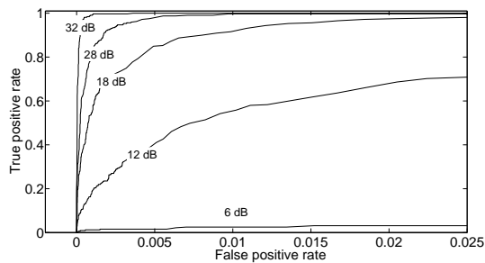
Figure 11: ROC of the duration-amplitude characterization.
