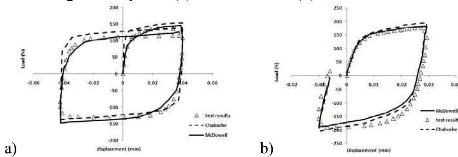
Fig. 4: Displacement controlled tests (a) Symmetric 10^{-2} mm/s at 180°C (b) Asymmetric 10^{-3} mm/s at 125°C.
