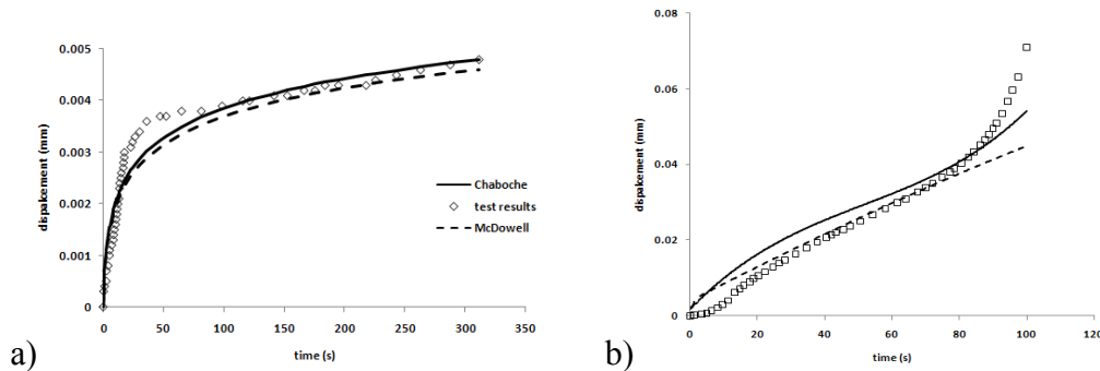
Fig. 3: Creep tests (a) 180N at 125°C (b) 120N at 180°C
