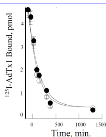
Figure 12. ^{125}I - \rho -Da1a ( ^{125}I -AdTx1) dissociation kinetics rate on \alpha 1aAR induced by 1 \mu M \rho -Da1a alone (open circles) or in addition with 1 \mu M prazosin (close circles).
