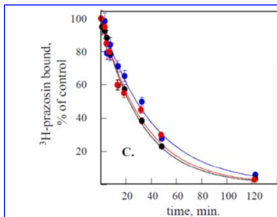
Figure 11. ^3H -prazosin dissociation kinetics rate on \alpha 1aAR induced by prazosin (1 \mu M , black) or \rho -Da1a (1 \mu M , blue) or both (red).
