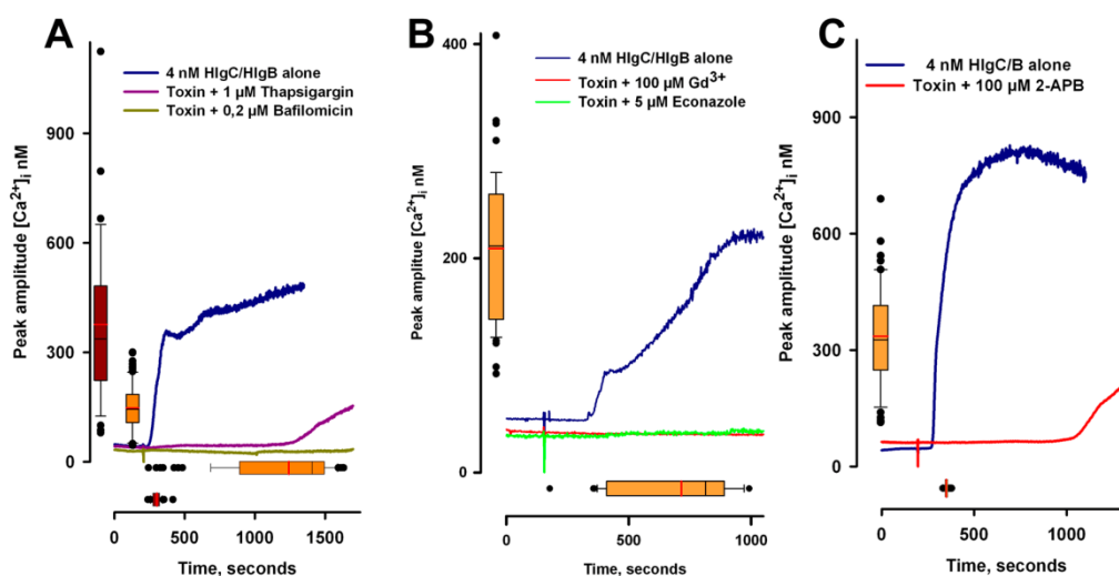
Figure 2. Contribution of intracellular Ca^{2+} stores to the leucotoxin HlgC/HlgB activity and antagonist effect of drugs active on the store operated calcium entry. (A) Incubation of neurons with 1 \mu M thapsigargin before addition of leucotoxin strongly inhibits the [Ca^{2+}]_i changes. Results are presented by a single trace, mean of all records from a same dish, and as box plots that present the median, the percentile and the mean as a red line. The box plots gather results from three experiments. (B) Blocking effect of Gd^{3+} and econazole and (C) of 2-APB; all drugs known to antagonize store operated calcium entry (SOCE). The same representation as in A is shown, except for SOCE antagonists where no [Ca^{2+}]_i changes were observed or they were extremely reduced.
