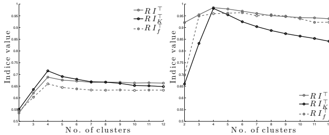
Figure 1. RI^\top(R, Q_c) , RI_K^\top(R, Q_c) and RI_f^\top(R, Q_c) for the data set (A), for c = 2, 12 , with \top_{H_0} (left) and \top_{H_{100}} (right)
