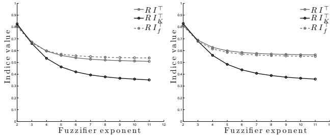
Figure 2. RI^\top(R, Q_m) , RI_K^\top(R, Q_m) and RI_f^\top(R, Q_m) for the data set ( B ), with different values of the fuzzifier exponent m = 2, 11 , with \top_{F_{0.1}} \rightarrow \top_M (left) and \top_{F_1} = \top_P (right)
