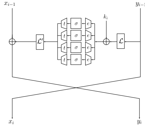
Fig. 2. Round i of \mathcal{KN}' -cipher
