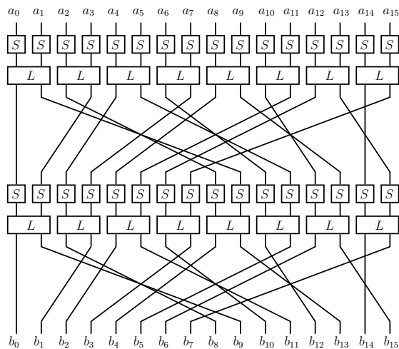
Fig. 4. Two rounds of R_4
