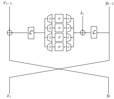
Fig. 2. Round i of \mathcal{KN}' -cipher
