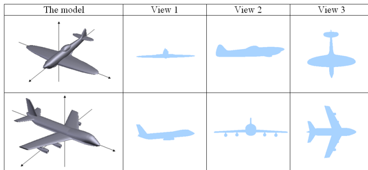
Figure 6: PCA miss-alignment. The choice of the principal axes is different for the two models with respect to their components which creates wrong matches (view 1 and view 2).
