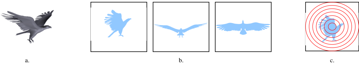
Figure 5: Principle of the PPD approach: a. the 3D model; b. the object's projections onto the principal planes; c. concentric circles used to determine the descriptor.
