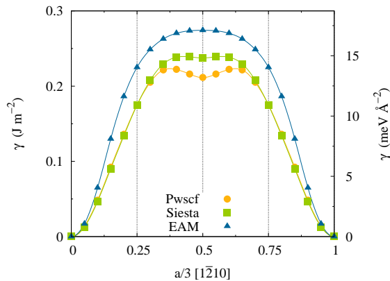
FIG. 4. Generalized stacking fault energy in the prism plane along the [1\bar{2}10] direction calculated with PWSCF, SIESTA and EAM potential.
