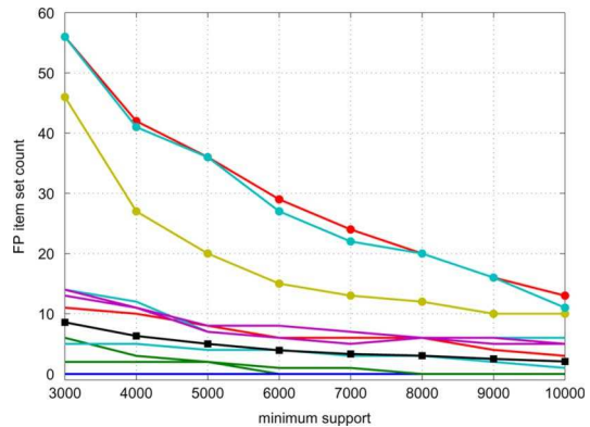
Fig. 9. Number of false positive (FP) item-sets generated by Apriori for different minimum support parameter values for 10 anomalous intervals (30%). For 21 anomalous intervals (70%), we obtain no FP item-sets at all. The average FP item-set count over all 31 anomalous intervals is marked with squares.
