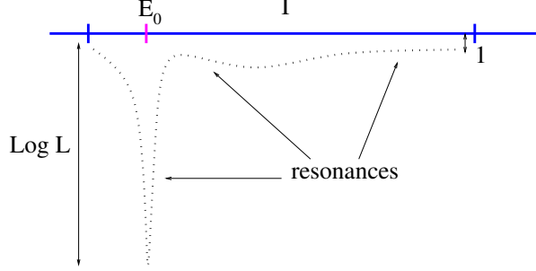
FIGURE 3. The resonances close to the real axis in the periodic case (after rescaling their imaginary parts by L )
