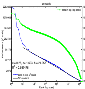
Figure 1: Stretched exponential distr. Fitting
