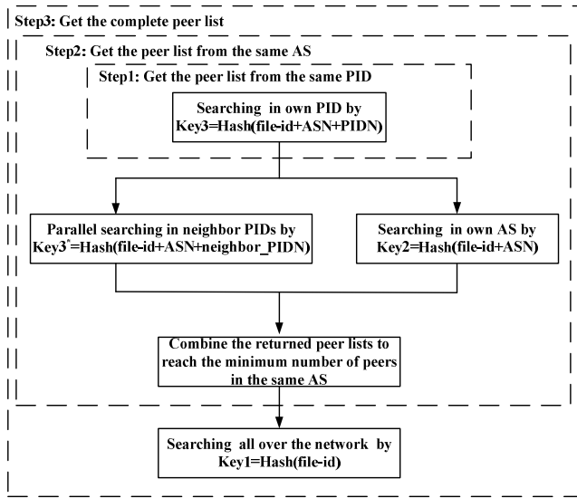
Fig. 4. Resource searching process for RP.
