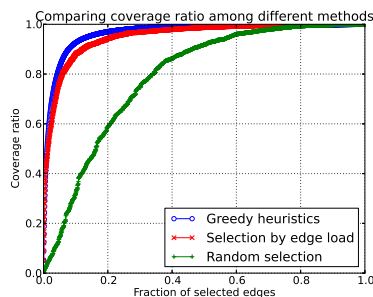
Fig. 3. Comparison of coverage ratio for different methods of selection
