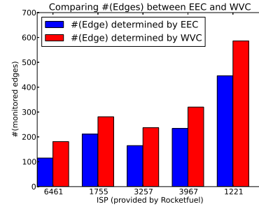
Fig. 2. Comparing number of monitored edges between EEC and WVC
