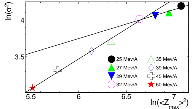
Figure 3: (color online) (Points) Log-log correlation between the first two cumulant moments ( \langle Z_{\max} \rangle^2 and \sigma^2 ) of the order parameter's distribution; (Lines) linear fits performed in the range 50-32 MeV/A (resp. 32-25 MeV/A) which correspond to a slope \Delta \sim 1 (resp. \Delta \sim 0.5 ) (see text).
