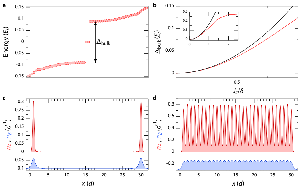
Figure 4. a. Spectrum of Bogoliubov excitations (red dots) for a homogeneous system with sharp boundaries, calculated for J_z = \delta , and J = 2\Delta^{(2)} . It exhibits a bulk gap \Delta_{\text{bulk}} = 0.18 E_r , and a pair of zero-energy Majorana states with a residual splitting \Delta_s \sim 10^{-12} E_r . b. Evolution of the bulk gap amplitude \Delta_{\text{bulk}} as a function of the ratio J_z/\delta (red line), for J = \Delta^{(2)} , with \Delta^{(2)} given by eq.(4). The black line represents the prediction of second-order perturbation theory \Delta_{\text{bulk}} = 2\Delta^{(2)} . c. Density distribution along x of a zero-energy Majorana state, in the planes A (red line) and B (blue line, offset for clarity). In the strong coupling regime J \sim \delta the population in B is not negligible. d. Total density distribution along x calculated at zero temperature. Majorana states are not visible in this almost uniform density profile.
