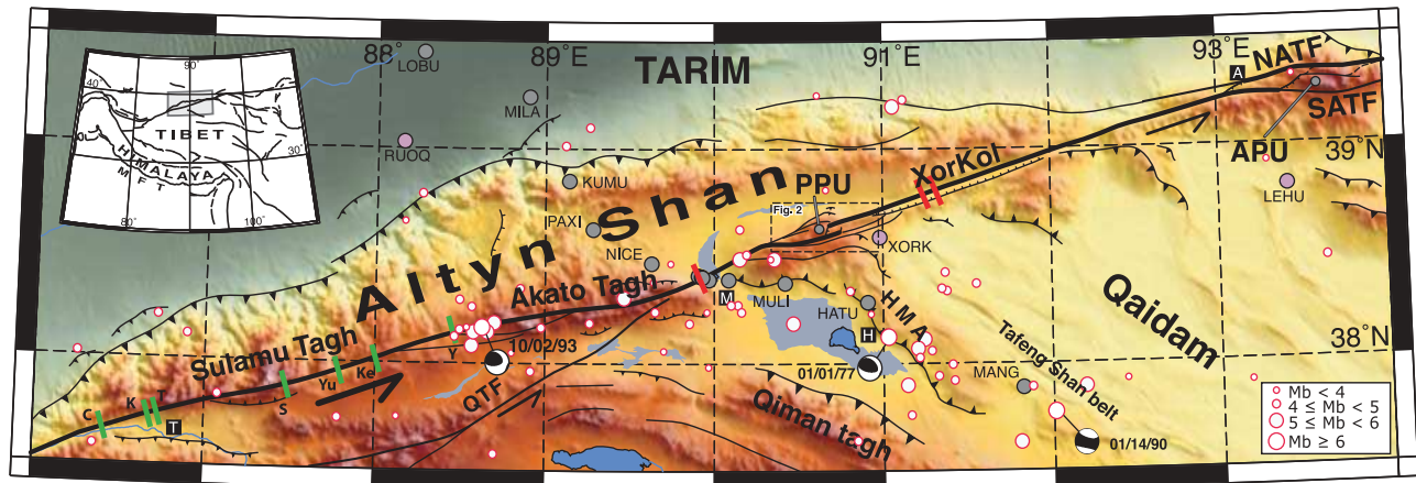
Figure 1. Map of topography and active faulting along Altyn Tagh Fault (ATF) system between 86° and 94°E. Mapping is based on field observations complemented by satellite imagery analysis and earlier work [e.g., Cowgill et al. , 2004a, 2004b; Mériaux, 2002; Meyer et al. , 1998; Tapponnier and Molnar, 1977; Tapponnier et al. , 2001]. SATF: South Altyn Tagh Fault, NATF: North Altyn Tagh Fault. Grey and purple dots are GPS stations from Bendick et al. [2000] and Wang et al. [2001], respectively. White dots are earthquakes from USGS/NEIC (PDE), with Harvard focal mechanisms for M_b \geq 6 . Thick green lines indicate published morphological sites at Cherchen He (C [Mériaux et al. , 2004; Cowgill, 2007]), Kelutelage (K [Gold et al. , 2011]), Tuzidun (T [Gold et al. , 2009]), Sulamu Tagh (S [Mériaux et al. , 2004]), Yukuang (Yu [Gold et al. , 2011]), Keke Qiapu (Ke [Gold et al. , 2011]) and Yuemake (Y [Cowgill et al. , 2009]). Thick red lines indicate trench locations of Washburn et al. [2003, 2001] (Kulesayi at \sim 90^\circ\text{E} and XorKol at \sim 91.25^\circ\text{E} ). A: Annamba, T: Tura, H: Huatugou and M: Mangnai Zhen. QTF: Qiman Tagh Fault [Tapponnier and Molnar, 1977], also named Kadzi Fault in Cowgill et al. [2004a]. HMA: Huatugou-Mangnai Anticlinorium. PPU and APU are Pingding Push-Up and Altyn Push-Up (gray lines), respectively. Lakes are in dark blue and salt flats are in pale blue. Studied sites are located along the main branch of the ATF in the Pingding Shan area between 90^\circ\text{E} and 91^\circ\text{E} . Dashed rectangle outlines area of Figure 2.
