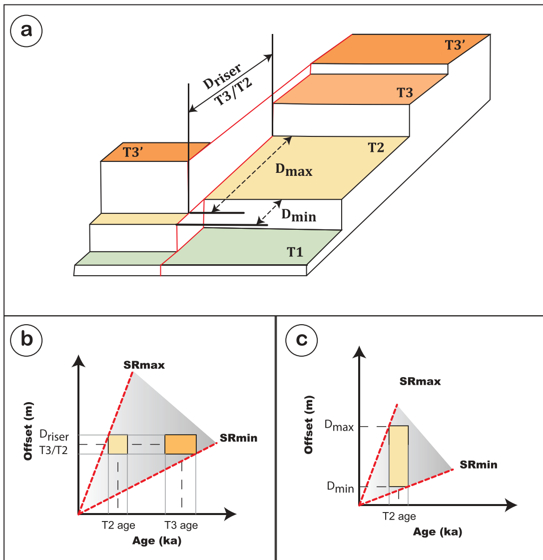
Figure 17. (a) Schematic 3D bloc diagram of terraces setting at site 1. D_{riser} is the offset of the T3/T2 riser, which may have accumulated after abandonment of T2 or after abandonment of T3. If the age of terrace thread T2 is considered, the extreme bounds of its offset range from D_{min} to D_{max} . (b) Slip-rate determination considering the uncertainty in the T3/T2 riser age. Bounds of riser age are the ages of the lower (T2) and upper terrace (T3) from which maximum and minimum rates, respectively, are derived. (c) Slip-rate determination considering the uncertainty in offset accumulation after abandonment of a given terrace. Bounds of the T2 terrace offset are the offsets of its upper T3/T2 and lower T2/T1 risers.
