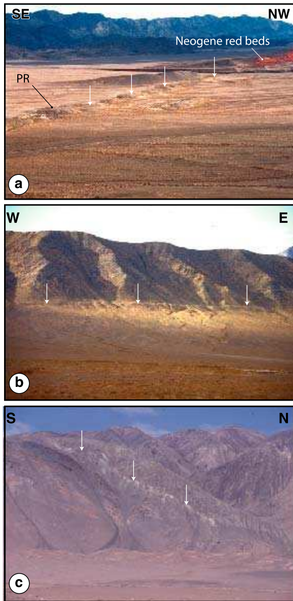
Figure 4. (a) North-looking view of cumulative pressure ridges along PDSF across \sim 800 m-wide fan (F) (see Figure 3). Note deformed Neogene red beds capped by south-dipping Quaternary conglomerates in background. PR points to one particularly large cumulative pressure ridge. White arrows point to active PDSF trace. (b) Shutter ridges, and stream channels offset by ATF main strand along Pingding range-front west of S2. Arrows indicate active trace of PDSF. (c) Northwestward-looking picture of the EPNF. Note the whitish fault trace showing a fresh rupture on a secondary fault ( N80^{\circ}E ) affecting the bedrock of the Pingding Shan.
