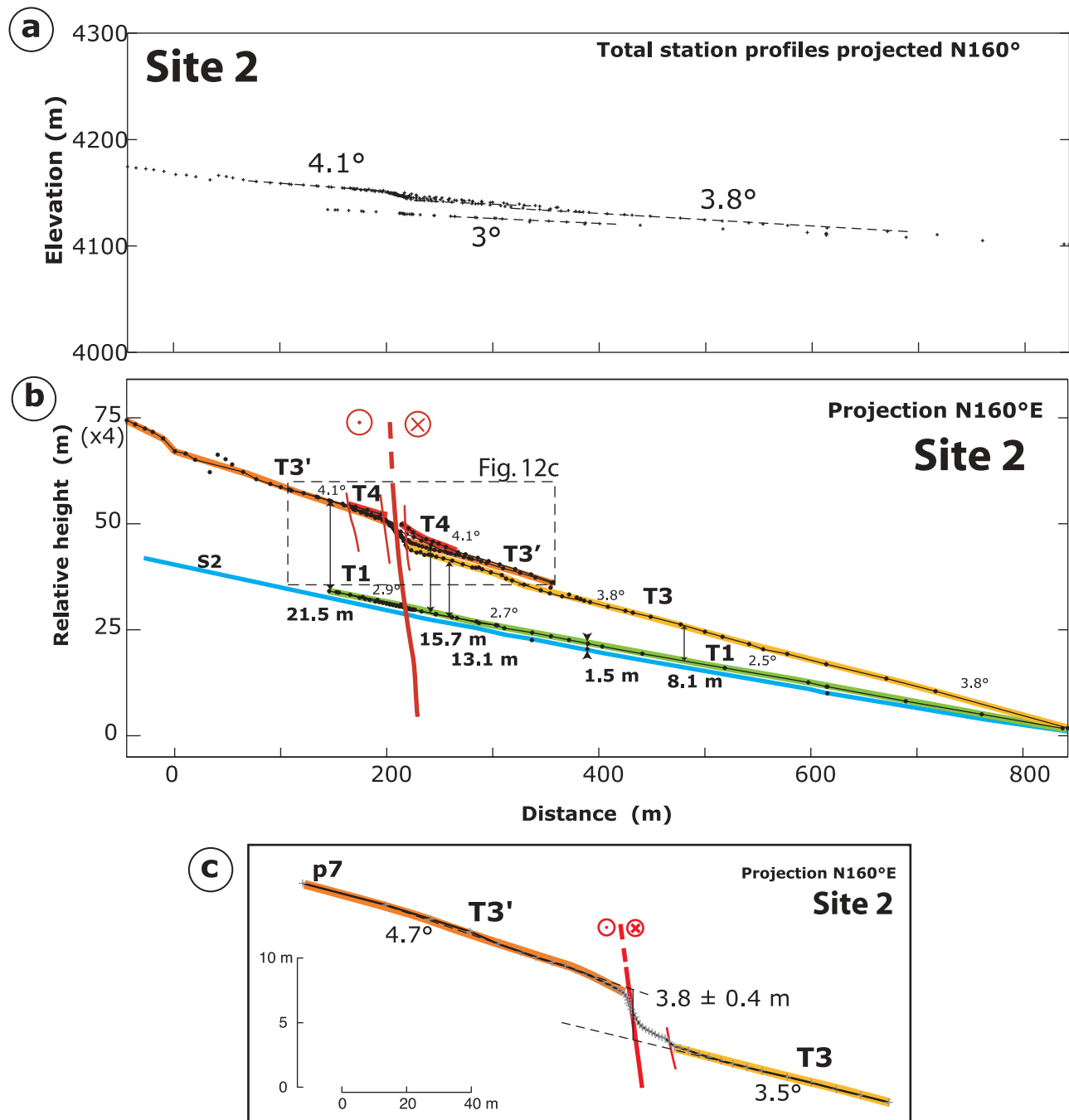
Figure 12. Site 2. Projection of total station profiles at high-angle to the fault on N160°-striking plane perpendicular to local fault strike. (a) Average south slope is indicated on 1 × 1 scale projection. (b) Projection with vertical exaggeration of four shows heights of terraces above streambed. Incision amounts are comparable to those at site 1 south of the fault, but are larger north of the fault due to local vertical displacements. (c) Height of steep main fault scarp separating T3' and T3 along profile p7 (see discussion in text).
