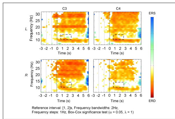
Fig. 1. Time-frequency maps displaying significant ERD (red) and ERS (blue) for Subject 6 (a typical example) in BCI competition IV IIB. The areas in the rectangles are the time-frequency areas selected by the proposed method. Imaginations of left and right hand movement elicited contrary contralateral dominant ERD in the selected areas, which indicates the effectiveness of the proposed method in time-frequency selection for discrimination.
