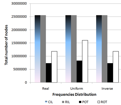
Figure 6: Impact of the distribution on index size
