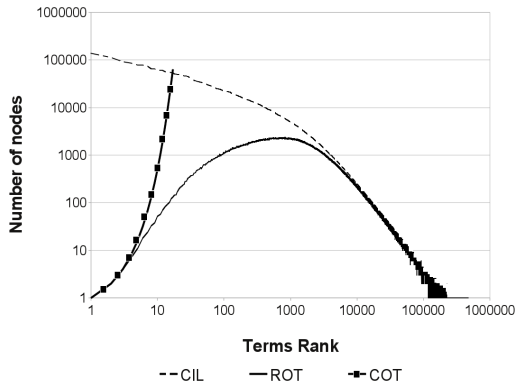
Figure 2: # nodes vs term’s rank
