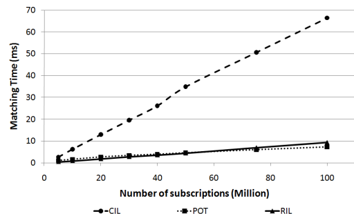
Figure 11: Matching time by scaling |\mathcal{S}|
