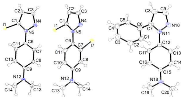
Figure 1 ORTEP diagrams (30% probability) of 2b (left), 3b (middle) and 4b (right).
