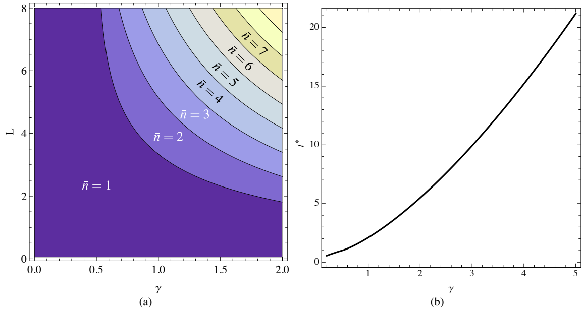
Fig. 9 Key properties of the solution of the static problem of a film of dimensionless length L and relative debonding toughness \gamma (see Proposition 4). (a) Plot of \bar{n} as a function of L and \gamma , \bar{n} being the minimum number of pieces into which the film is split by transverse fractures when debonding appear (b) Plot of t^* as a function of the relative debonding toughness \gamma , t^* being the critical load beyond which the optimal solution is that of a debonded film without transverse fractures ( t^* is independent of the dimensionless length L of the film).
