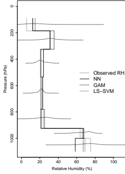
Figure 2: Example of Estimation of relative humidity profile. The observed profile is the thick gray line and the 3 estimations (plain(NN), dashed(GAM), dots(LS-SVM)) are in black. Conditional density distribution estimated from GAM model errors are showed for each layer (dashed) using Mixture Gaussian Model with m=2
