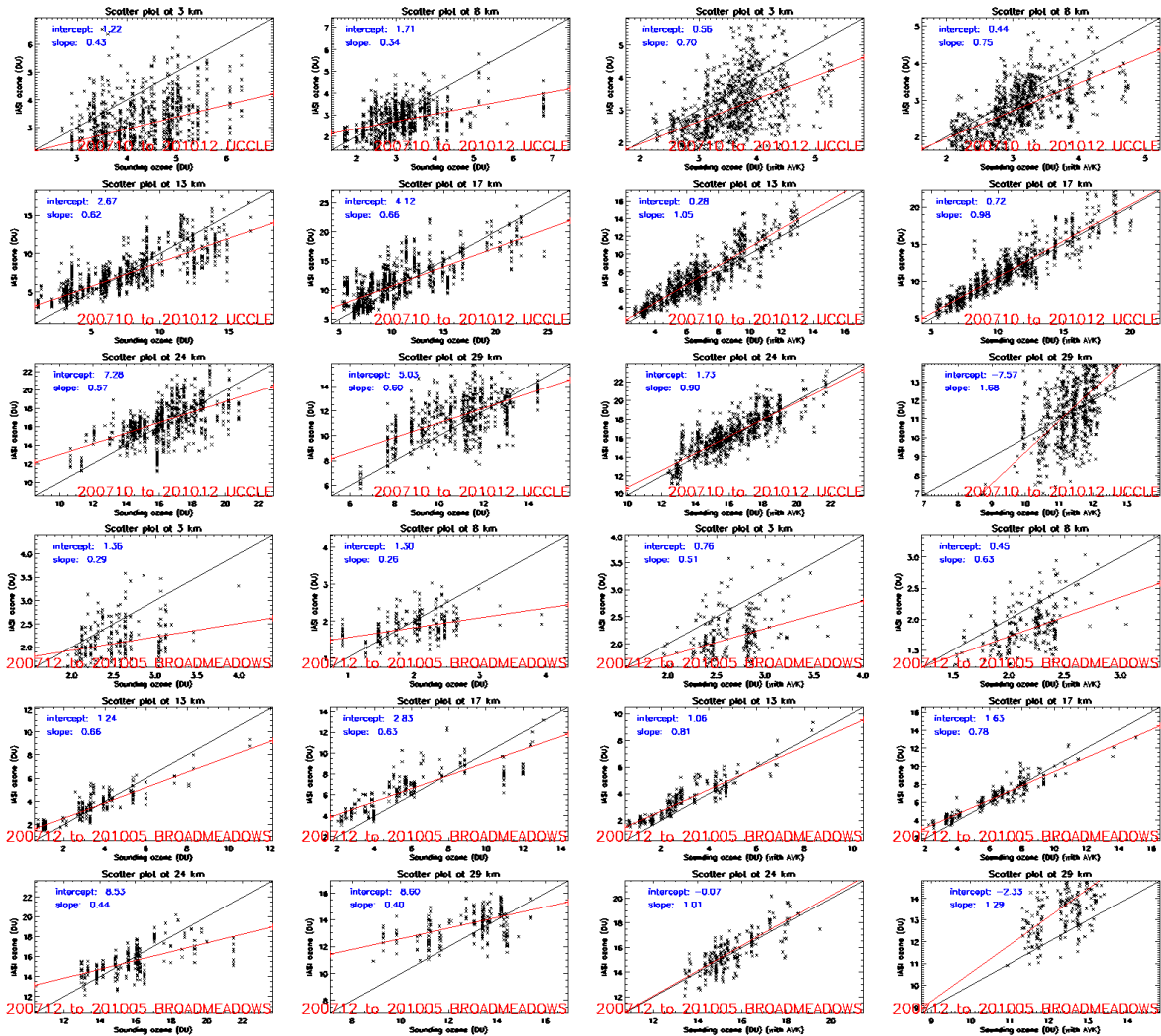
Figure 3: Scatter plot at 6 different altitude levels for the stations of Uccle and Broadmeadows. (left: IASI <-> ozone sonde, right: IASI <-> smoothed ozone sonde)
