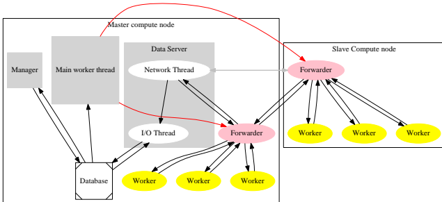
FIG. 3: Overview of the QMC=Chem architecture.
