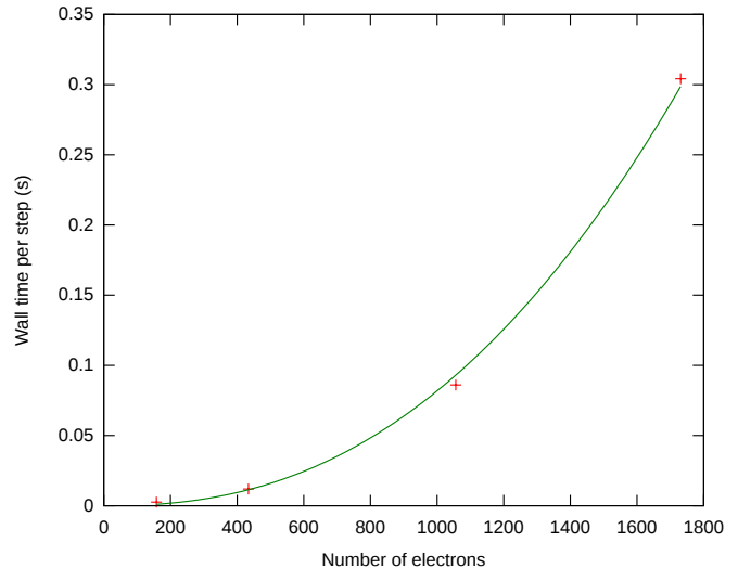
FIG. 2: Single-core scaling with system size.
