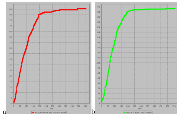
Fig. 6. a. The figure shows the average time that one agent spends from his initial position to the target. At the time step 555, the average time converges 85 steps. b. The figure represents the number of agents that reach the targets. At the time 555, the number of agent reach the target is converges 460 agents
