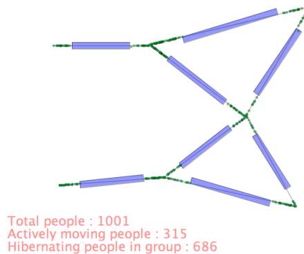
Fig. 8. Micro model of the road networks and Hybrid model of road networks are implementation. The number of people hibernating (not simulated in the ABM) are proportional to the speedup provided by the hybrid modeling. Indeed, only the fraction of the total pedestrians are effectively consuming simulation CPU.
