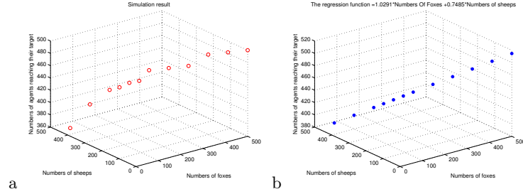
Fig. 7. The above result uses a constant mean velocity 10 m/7.5 seconds and variance velocity 1 m/7.5 seconds. a. a shows the simulation result of the number of agents reaching the targets. b. shows an analysis result of the agents reaching the target by using the linear regression.
