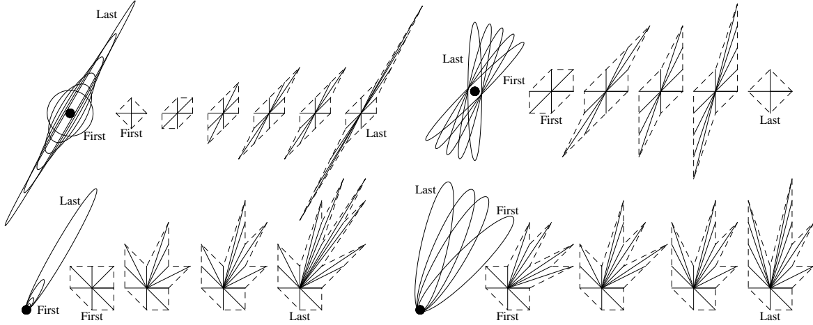
Figure 3: Top : the mesh \mathcal{T}(F) constructed for norms F of anisotropic euclidean type (i.e. F(u) := \sqrt{u^T M u} for some matrix M \in S_2^+ ), of anisotropy ratio \kappa(F) ranging from 1 to 32 and orientation \pi/3 (top left), or of anisotropy ratio \kappa(F) = 10 and orientation ranging from \pi/4 to \pi/2 (right). Bottom : likewise for asymmetric norms of the form F(u) := \|u\| - \langle \omega, u \rangle , u \in \mathbb{R}^2 , of anisotropy ratio ranging from 4 to 400 and orientation \pi/3 (bottom left), or of anisotropy ratio 100 and varying orientations (bottom right).
