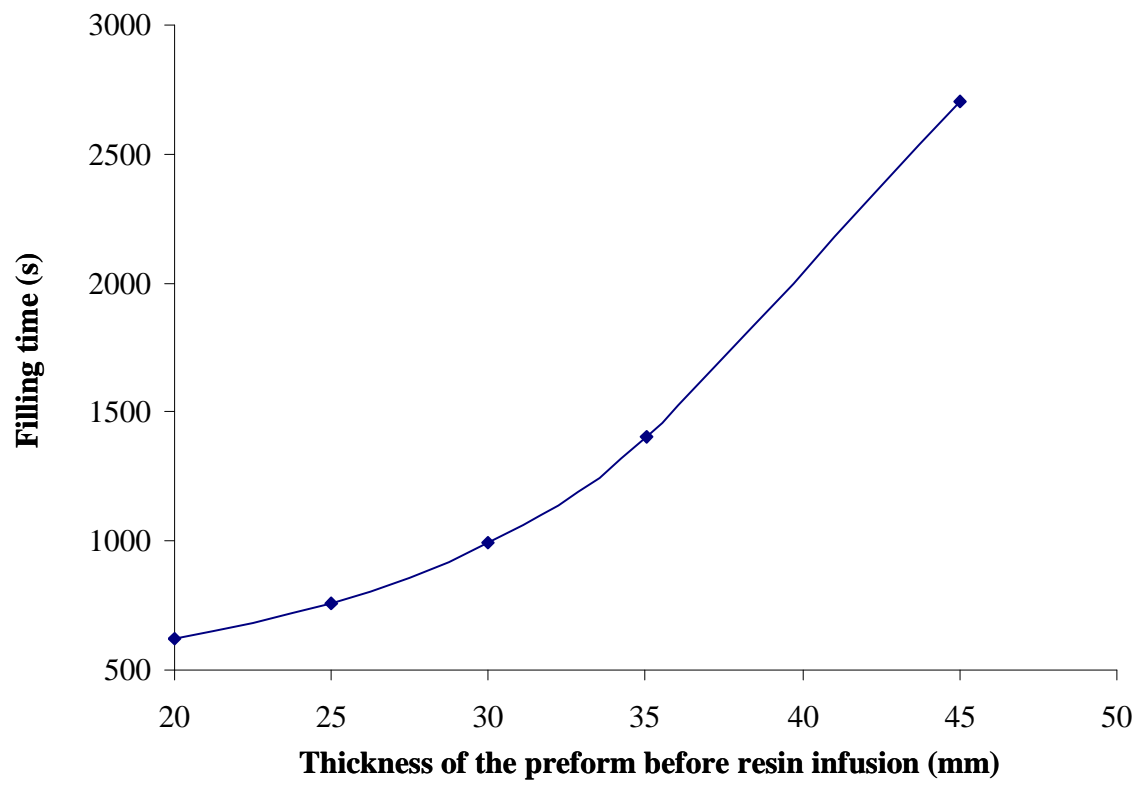
Fig. 5. Changes in the filling time vs. the initial thickness of the preform
