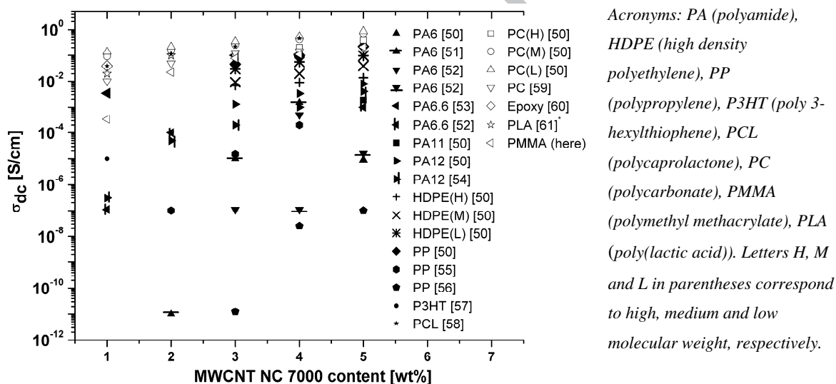
Figure 5. Conductivity values ( \sigma_{dc} ) at various MWCNT contents for several conducting polymer systems prepared using the same type of MWCNT (Nanocyl NC 7000). Open (right column in the legend) and solid symbols (left column in the legend) signify amorphous and semicrystalline systems, respectively.
