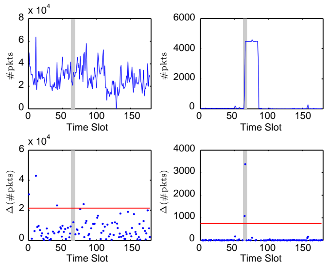
Figure 2: Low-intensity anomalies might be hidden inside highly aggregated traffic, but are visible at finer-grained aggregations. The DDoS attack is evident at the victim’s network.
