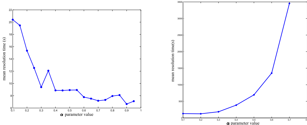
Figure 10: Evolution of the resolution time with respect to the \alpha parameter of the sphere (left) and the box (right) examples.
