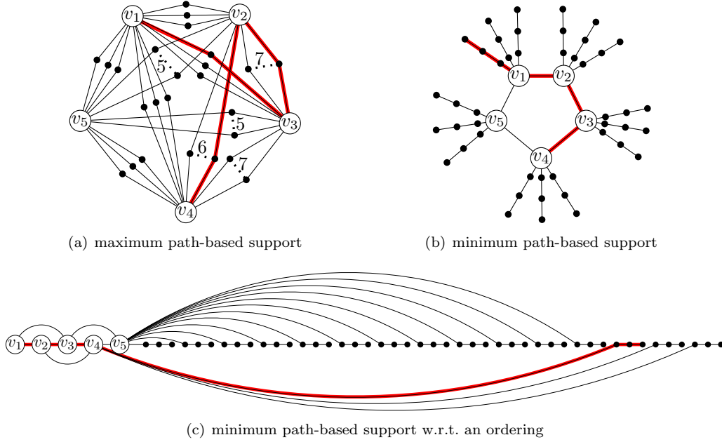
Figure 4: Three different supports for the hypergraph H_I introduced in Section 3.1. The small black vertices are the vertices v_{\sigma,x} , \sigma \in I , x = 1, 2, 3 . The thick red path indicates the hyperedge h_{1324} .
