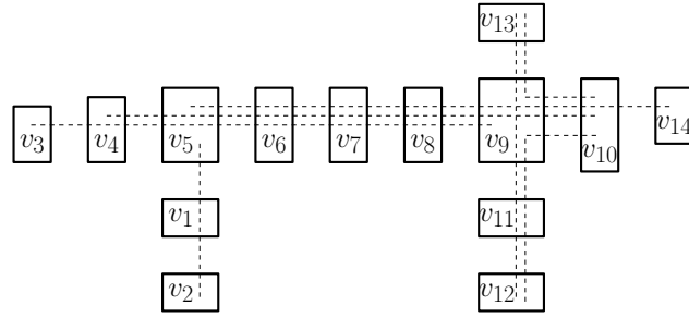
(f) metro map like drawing of the sources of D'
