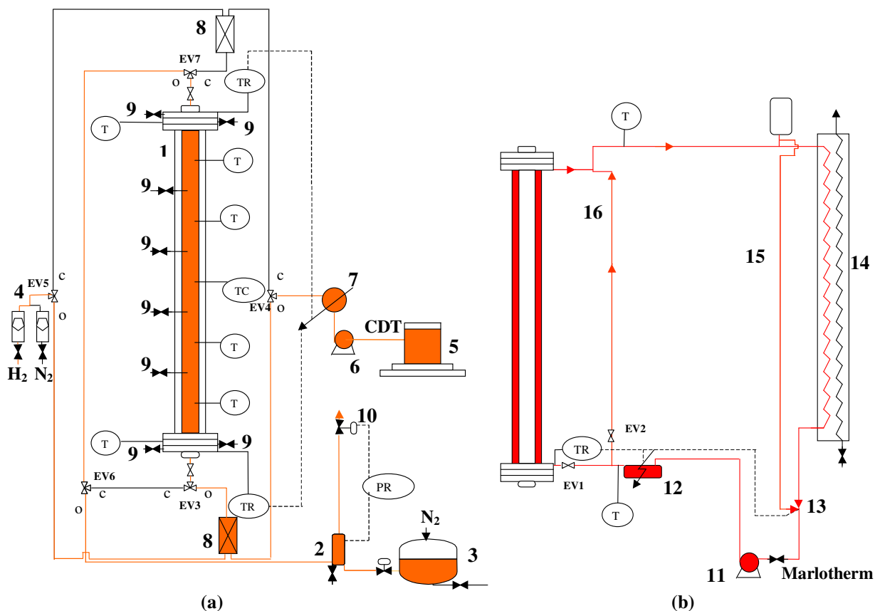
Fig. 1 – Experimental set-up: (a) reactant circuit (up-flow mode), (b) thermal control equipment.
