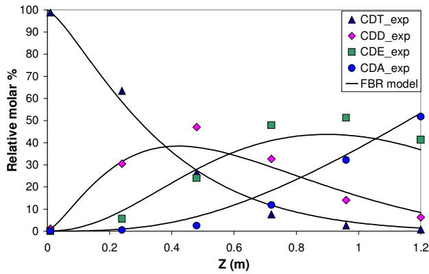
Fig. 8 – Axial concentration profiles in the flooded-bed ( P = 4 bars, T_{Me} = 100^{\circ}\text{C} , u_{Le} = 0.53 \times 10^{-3} m/s, u_{Ge} = 0.042 m/s).
