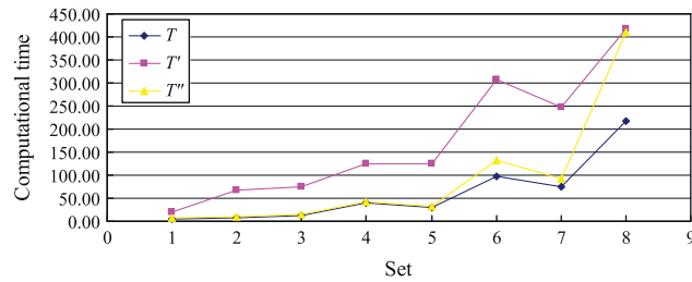
(a) Computational time T , T' and T''
