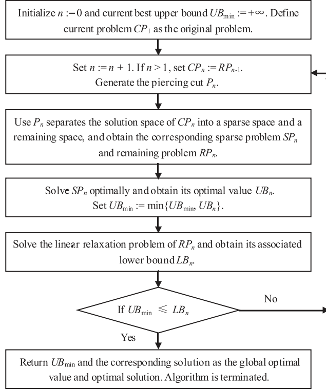
Fig. 2. Principle of the cut-and-solve method.
