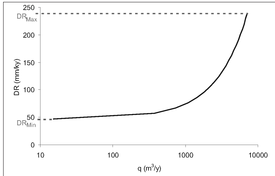
Fig. 3 – Principle of equation (7). Denudation rate of the topography DR is taken to be proportional to the underground flow q (subcutaneous zone).
