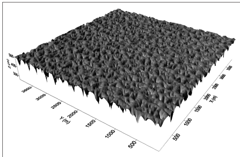
Fig. 5 – Example of a simulated cockpit karst landscape. Here, the climatic factor is 2 and the simulation time is 4 My. The DEM of a simulated landscape can be used to perform analysis. In this study, three analyses are carried out: average slope, relative relief and scaling characteristics.
