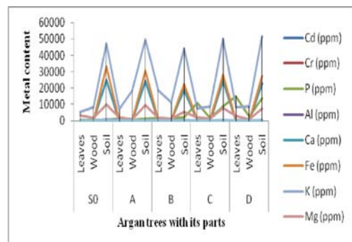
Fig. 2 Representation of different levels of heavy metals and micronutrients in wood, leaves and soil of the argan tree (23/10/08)
