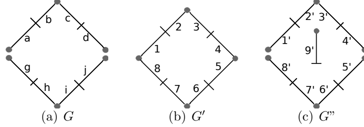
Figure 4: Examples of non isomorphic maps for which the distance may be null. d_{\omega_1,0}^p(G, G') = 0 because G \sqsubseteq^p G' and G and G' have the same number of darts. However G and G' are not isomorphic. Therefore d_{\omega_1,0}^p is not a metric. Also, d_{0,\omega_2}^*(G, G'') = 0 because G \sqsubseteq^p G'' and G and G'' have the same number of seams (dart 9 is not sewn). However G and G'' are not isomorphic. Therefore d_{0,\omega_2}^* is not a metric.
