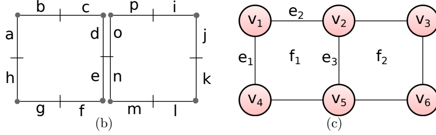
Figure 1: Example of 2G-map. (a) describes \alpha_i involutions of a 2G-map composed of 16 darts denoted by letters from a to p . (b) displays a graphical representation of this 2G-map: darts are represented by grey segments labelled with the associated letter; incident darts separated by little black segments are 0-sewn (e.g., \alpha_0(b) = c and \alpha_0(c) = b ); incident darts separated with a dot are 1-sewn (e.g., \alpha_1(a) = b and \alpha_1(b) = a ); adjacent darts are 2-sewn (e.g., \alpha_2(d) = o and \alpha_2(o) = d ). (c) displays the plane graph modelled by the 2G-map: vertices, edges, and faces of this graph correspond to sets of darts of the 2G-map (e.g., vertex v_1 corresponds to darts \{a, b\} , vertex v_2 to darts \{c, d, o, p\} , ..., edge e_1 to darts \{a, h\} , edge e_3 to darts \{d, e, o, n\} , ..., face f_1 to darts \{a, b, c, d, e, f, g, h\} , and face f_2 to darts \{i, j, k, l, m, n, o, p\} ).
