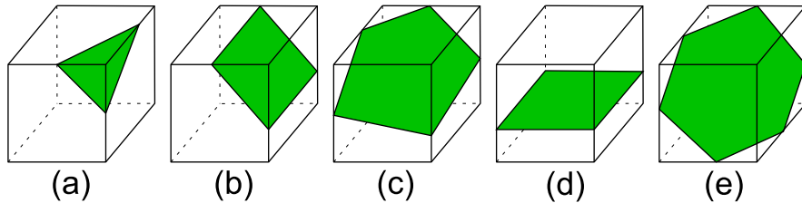
Figure 4: The five different shapes of convexels, which are constructed as the intersections between a rotation plane and voxels [12].
