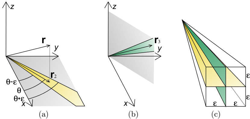
Figure 9: Example of the approximation of a 3D vector using our method. (a) and (b) represent the projections of \mathbf{r} into \mathbf{r}_2 and \mathbf{r}_3 in 2D planes respectively. Each 2D convex cone in (a) and (b) is the admissible approximation for \mathbf{r}_2 and \mathbf{r}_3 regarding to \epsilon . (c) represents the square pyramid constructed from the two 2D convex cones that contains the set of admissible approximations for \mathbf{r} .
