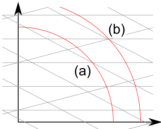
Figure 7: the two impossible cases of intersection between a circle centered on a grid point and a rational multi-grid.
