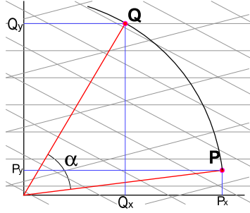
Figure 8: A hinge angle \alpha for a point \mathbf{p} in a rational multi-grid.
