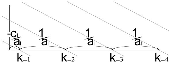
Figure 3: Parallel lines of a set \mathcal{L}_i and geometric interpretation of their parameters
