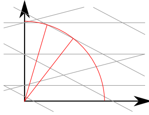
Figure 10: In a rational multi-grid \mathcal{M}^{A, a_i} a convexel can have four intersections with the locus of rotation of \mathbf{p} .
