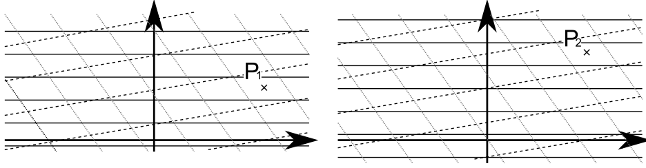
Figure 5: Two multi-grids generated by a rotation axis but with two different points \mathbf{p}_1, \mathbf{p}_2 one of which is obtained by a translation of \pm(\mathbf{p}_1 - \mathbf{p}_2) from the other.
