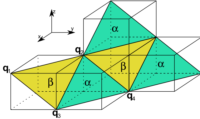
Figure 6: A quadruple of grid points \{\mathbf{q}_1 = \mathbf{q}, \mathbf{q}_2 = (q_x + A_x, q_y + A_y, q_z)^\top, \mathbf{q}_3 = (q_x + A_x, q_y, q_z - A_z)^\top, \mathbf{q}_4 = (q_x + 2A_x, q_y + A_y, q_z - A_z)^\top\} forms two types of triangles, \alpha and \beta tiled in a multigrid.
