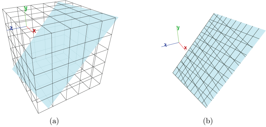
Figure 2: The 3D half-grid cut by a plane (a), and its multi-grid (b).
