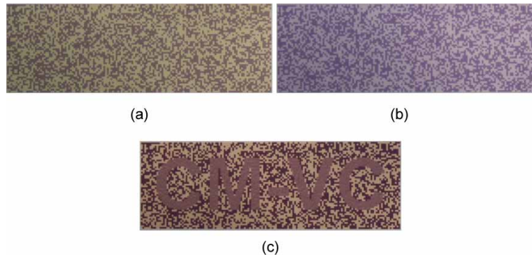
Fig. 6. An example of the proposed CM-VCS for which the secret message “CM-VC” is a desaturated red. There is no information about the secret message on each transparency (a) and (b). The secret content together with the color are revealed in transmission mode when the two transparencies are superposed (c) by using daylight illumination.
