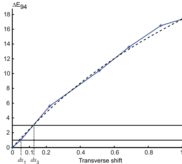
Fig. 8. Evolution of the color distance \Delta E_{94} for target color E with respect to a transverse shift (given in fraction of the size of a halftoned share) of one of the SIs. The blue curve corresponds to measurements of the spectral transmittance of the stack. The dashed curve corresponds to a mean spectral transmittance of such a superposition computed according to Eq. (8). When the transverse shift distance is zero, the distance \Delta E_{94} is null, and the stack color corresponds to target color E . When the transverse shift distance is 1, the color is completely different from the target color E . Below a shift dx_1 < 0.1 , the \Delta E_{94} value between target color E and the stack color is less than 1, i.e. the color difference cannot be perceived. Beyond the distance dx_3 , the \Delta E_{94} value is higher than 3, and a color difference is well perceptible.
