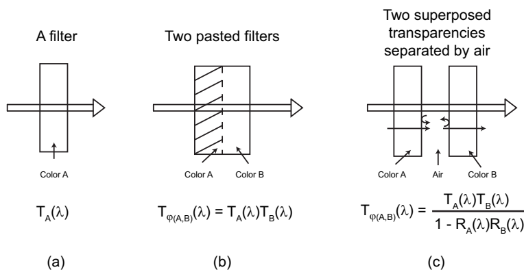
Fig. 4. (a) Transmittance of a filter. (b) Transmittance through two superposed filters without taking into account the air slice between them. (c) Transmittance of two superposed transparencies separated by a thin air slice.
