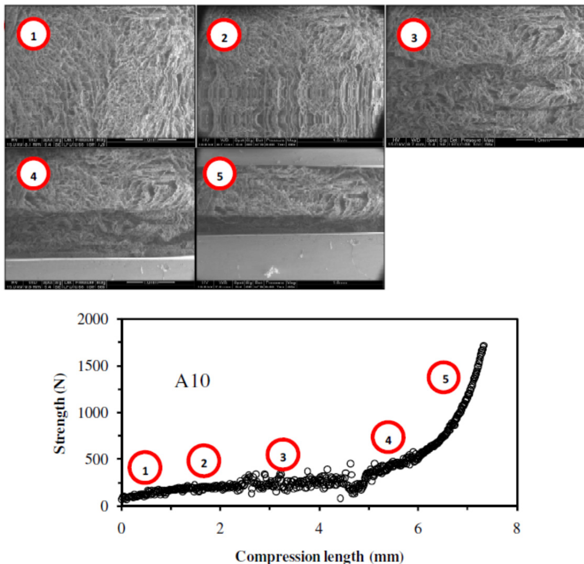
Figure 4. Compression test of A10 catalytic material: SEM observations and evaluation of mechanical characteristics.
