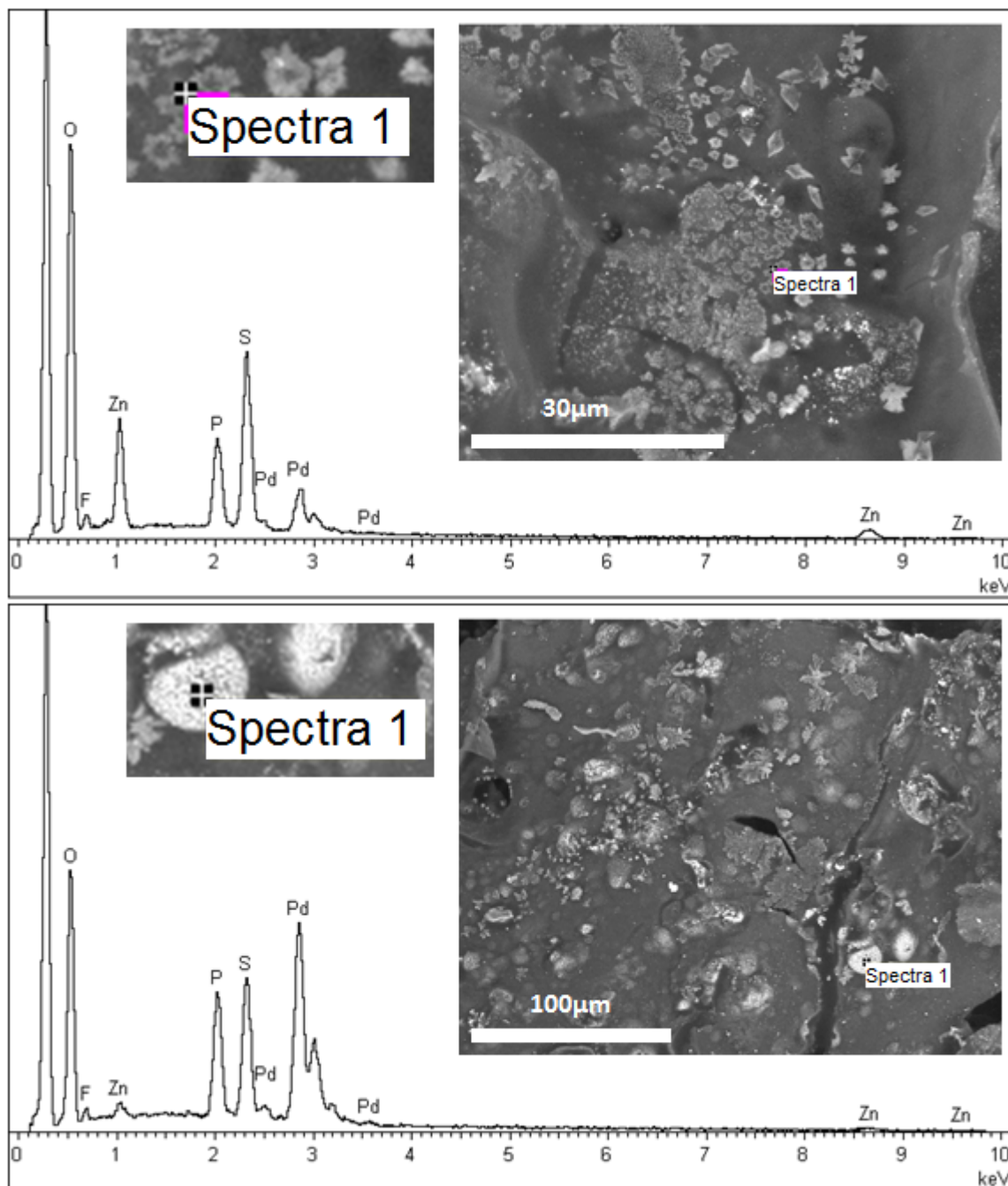
Figure 2. SEM-EDX analysis of specific zones of A3 catalytic material: focuses on white areas (Spectra 1).
