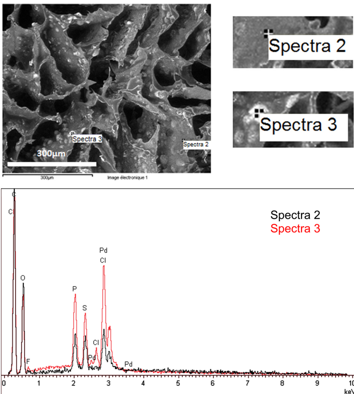
Figure 1. SEM-EDX analysis of specific zones of A1 catalytic material: focus on a non-specific zone (grey area, Spectra 2) and on an IL vesicle (white area, Spectra 3).
