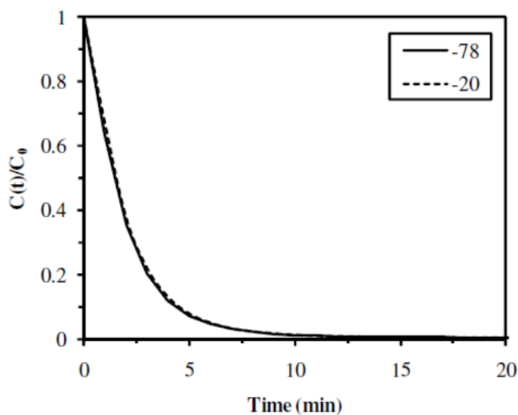
Figure 6. Influence of freezing temperature on the catalytic hydrogenation of 4-NA (Catalytic materials: A1 (T: -78\text{ }^{\circ}\text{C} ), and A2 (T: -20\text{ }^{\circ}\text{C} )).
