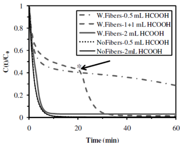
Figure 10. Impact of the presence of cellulose fibers and amount of formic acid on the catalytic hydrogenation of 4-NA (Catalytic materials: A1 (NoFibers) and A10 (W.Fibers); * supplementary addition of a 1-mL volume of formic acid).
