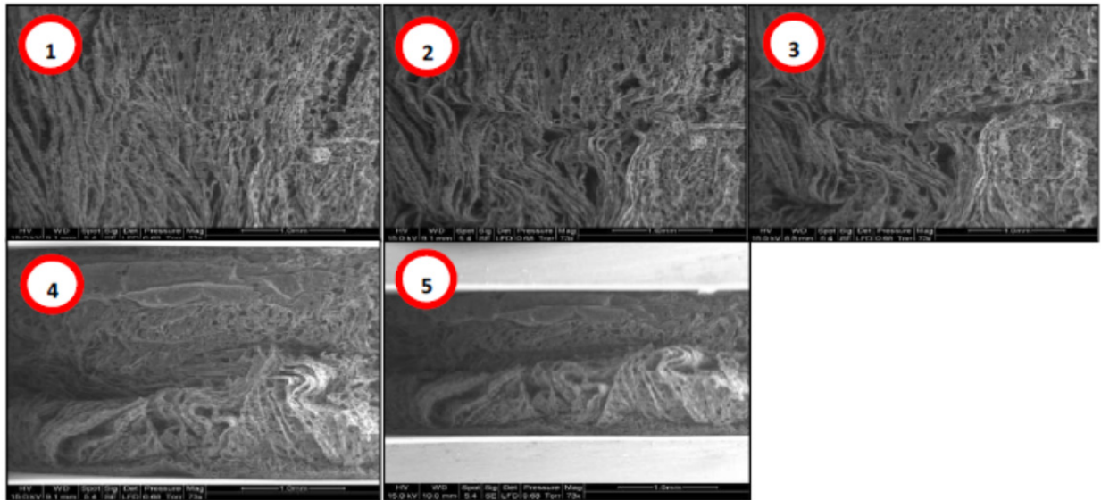
Figure 3. Compression test of A1 catalytic material: SEM observations and evaluation of mechanical characteristics.
