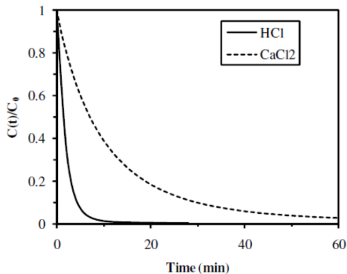
Figure 8. Influence of the type of gelation of the materials on the catalytic hydrogenation of 4-NA (Catalytic materials: A1 (0.5 M HCl) and A3 (0.4 M CaCl 2 )).
