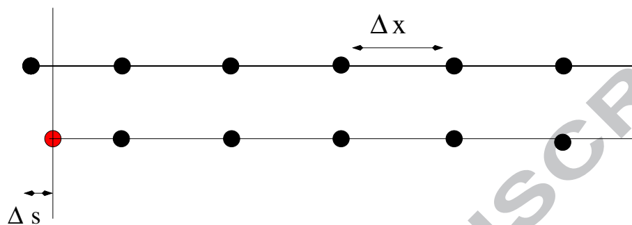
Figure 1: Due to surface sublimation a certain amount of material is ejected from the surface of the nucleus. This leads to a moving boundary and to a deviation between the actual grid and the current position of the surface. Special techniques are necessary for a proper treatment.
