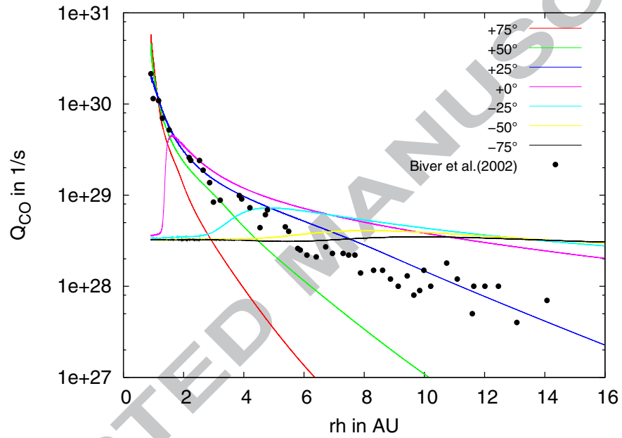
Figure 5: Similar CO plot as in Fig. 4 for the post-perihelion branch. The CO data of Biver et al. [2002] along the post-perihelion branch could be fitted if CO activity is confined to the positive hemisphere above a latitude of +10^\circ as in the pre-perihelion case of Fig. 4.
