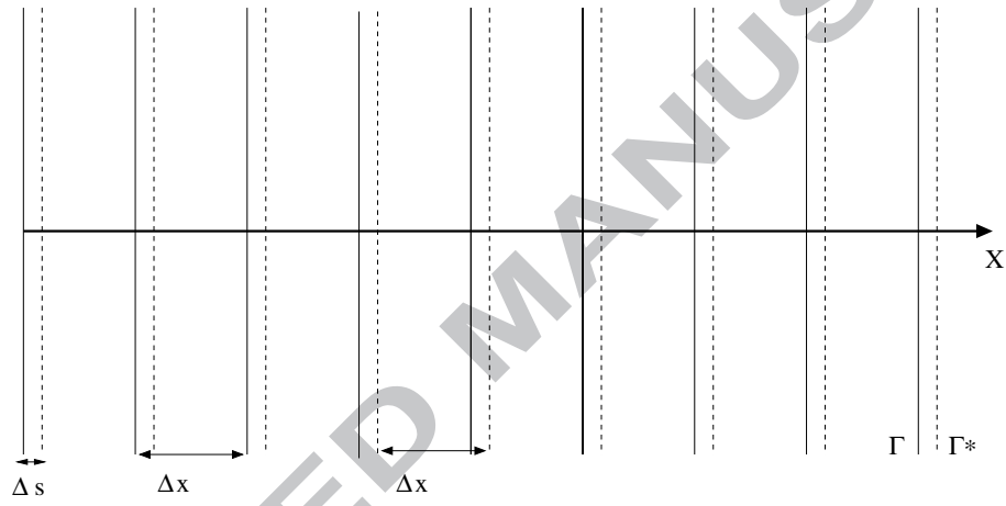
Figure 2: The spatial discretization size \Delta x remains constant throughout the computation. The old grid \Gamma is moved according to the erosion of surface material \Delta s . The temperature field at the new grid \Gamma^* is obtained through interpolation with cubic splines [Crank and Gupta , 1972].
