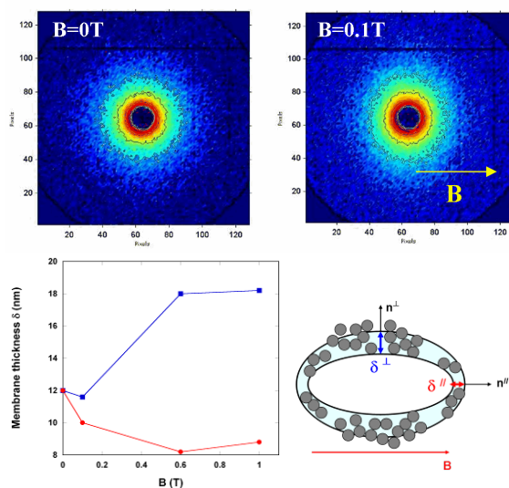
Fig. 2 Top: SANS patterns of magnetic vesicles loaded at 50 wt. % MNPs in H 2 O in the q range 3 \times 10^{-3} - 3 \times 10^{-2} \text{ \AA}^{-1} at zero field and under B=0.1 Tesla. Colors correspond to iso-intensity ranges. Patterns were averaged in angular sectors ( -30^{\circ} 30^{\circ} ) along the field direction or ( -15^{\circ} 15^{\circ} ) around the perpendicular direction. Bottom: Kratky-Porod fits \text{Ln}[q^2 I(q)] \sim -q^2 \delta^2 / 12 in the low q regime lead to membrane thicknesses in the two directions \delta^{\parallel} and \delta^{\perp} and to a scheme of the overall deformation.
