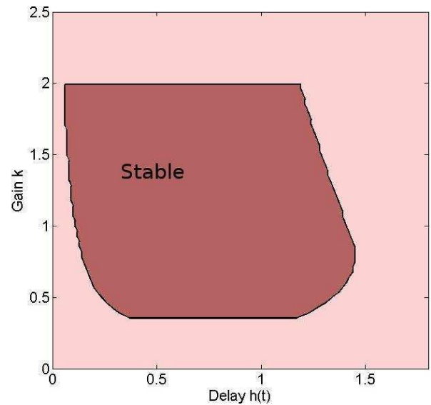
Fig. 2. Stability region of \ddot{y}(t) - 0.1\dot{y}(t) + 2y(t) = ky(t - h(t)) w.r.t. k and h(t) .
