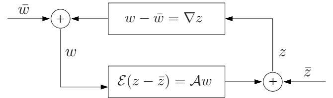
Fig. 1. Feedback system.
